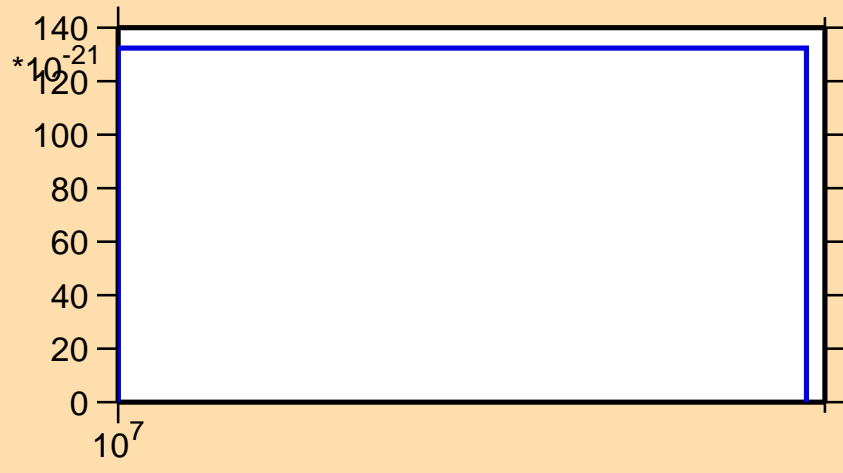
\sigma vs. E for ^{148}\text{Nd}(\text{mt } 11)
