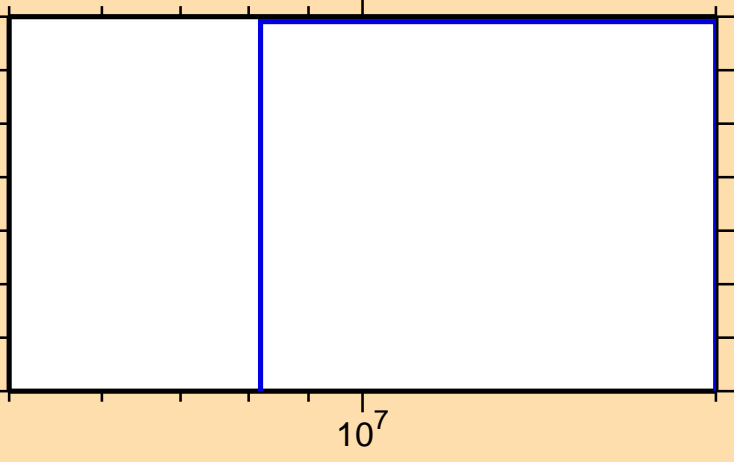
\sigma vs. E for ^{148}\text{Nd}(n,2n\alpha)
