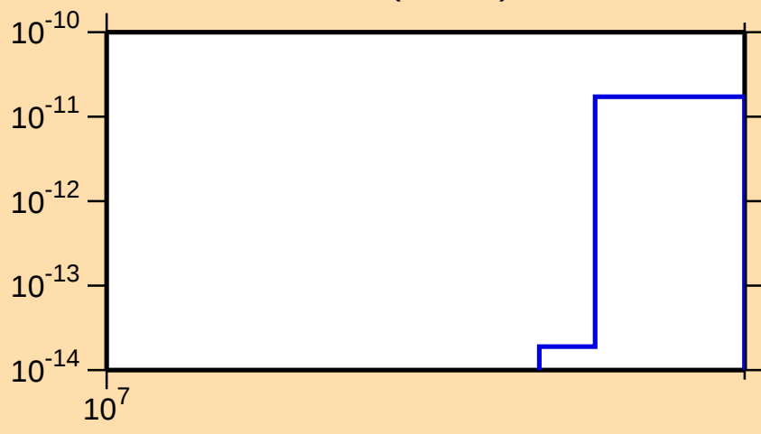
\sigma vs. E for ^{149}\text{Nd}(n,3n\alpha)
