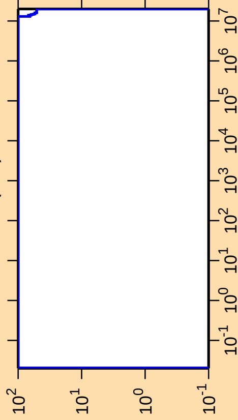
\Delta\sigma/\sigma vs. E for ^{149}\text{Nd}(n,\alpha)
