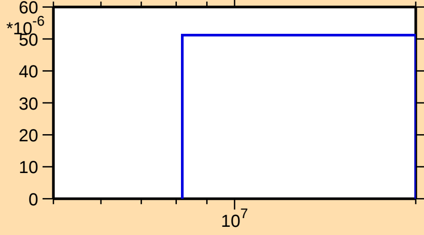
\sigma vs. E for ^{149}\text{Nd}(n,np)
