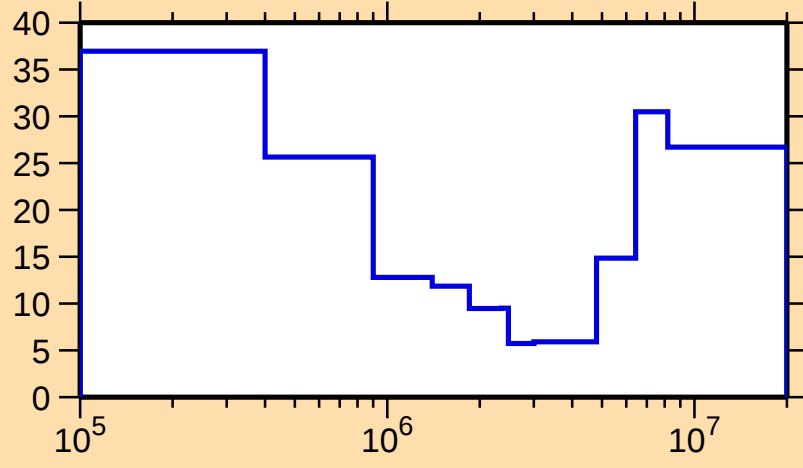
\Delta\sigma/\sigma vs. E for ^{149}\text{Nd}(n,\text{inel.})
