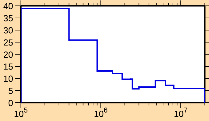
\Delta\sigma/\sigma vs. E for ^{149}\text{Nd}(n,\text{nonel.})
