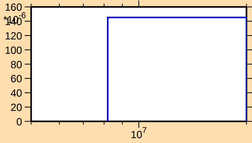
\sigma vs. E for ^{149}\text{Nd}(n,d)
