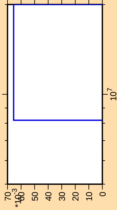
\Delta\sigma/\sigma vs. E for ^{149}\text{Nd}(n,\text{He}3)
