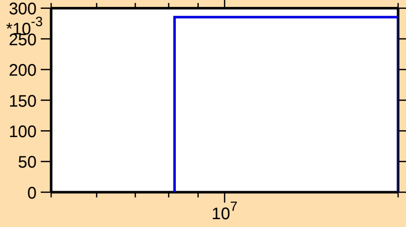
\sigma vs. E for ^{149}\text{Nd}(n,3n)
