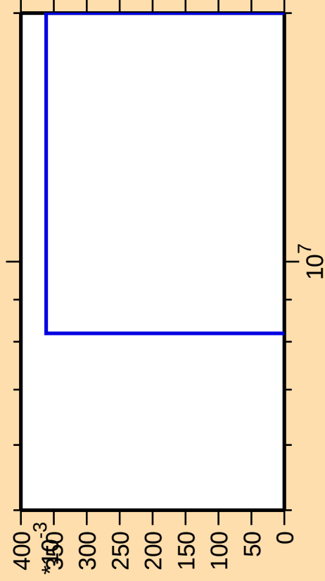
\Delta\sigma/\sigma vs. E for ^{149}\text{Nd}(n,3n\alpha)
