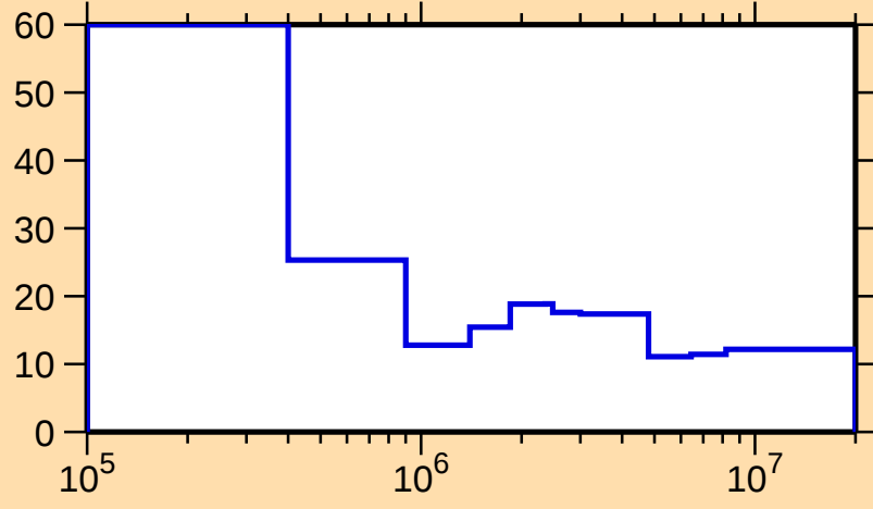
\Delta\sigma/\sigma vs. E for ^{149}\text{Nd}(n,\text{el.})
