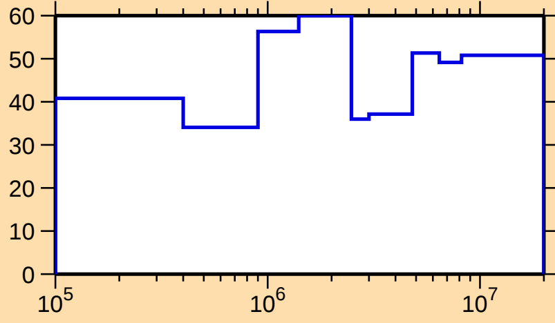
\Delta\sigma/\sigma vs. E for ^{149}\text{Nd}(n,n_1)
