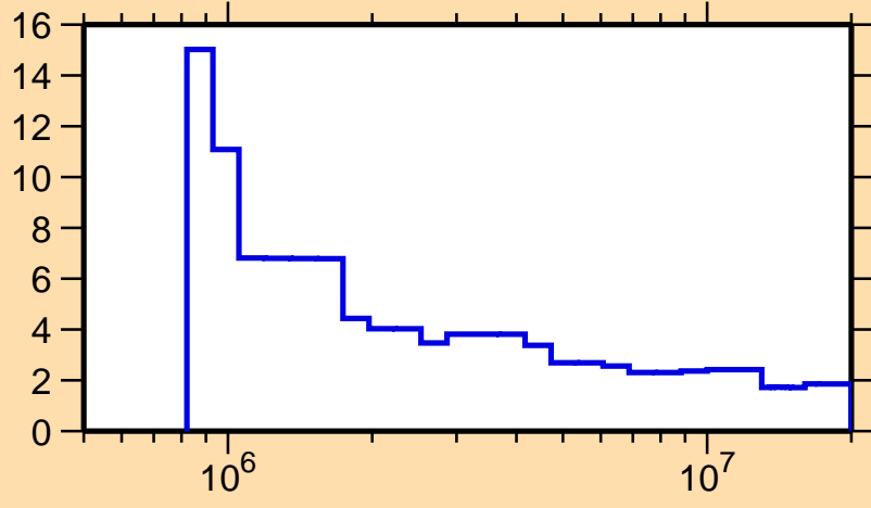
\Delta\sigma/\sigma vs. E for ^{151}\text{Nd}(n,\text{nonel.})
