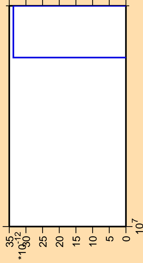
\Delta\sigma/\sigma vs. E for ^{151}\text{Nd} (mt 11)
