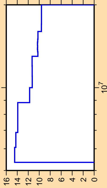
\Delta\sigma/\sigma vs. E for ^{151}\text{Nd}(n,n_1)
