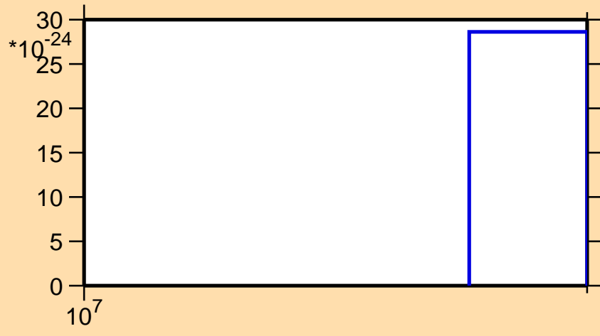
\sigma vs. E for ^{151}\text{Nd} (mt 11)
