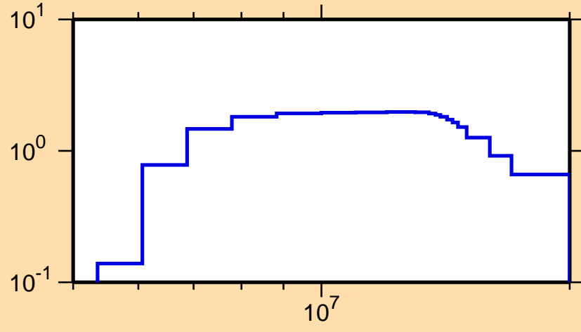
\sigma vs. E for ^{151}\text{Nd}(n,2n)
