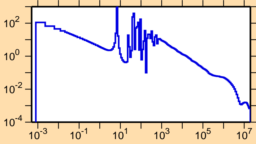
\sigma vs. E for ^{151}\text{Nd}(n,\gamma)
