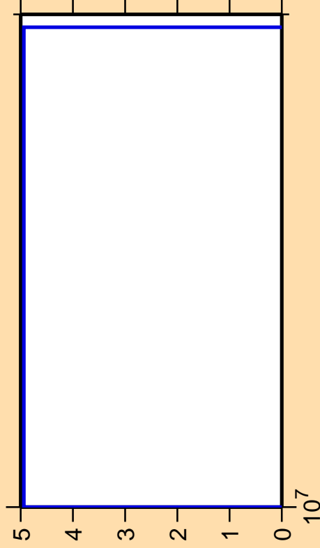
\Delta\sigma/\sigma vs. E for ^{151}\text{Nd}(n,3n)
