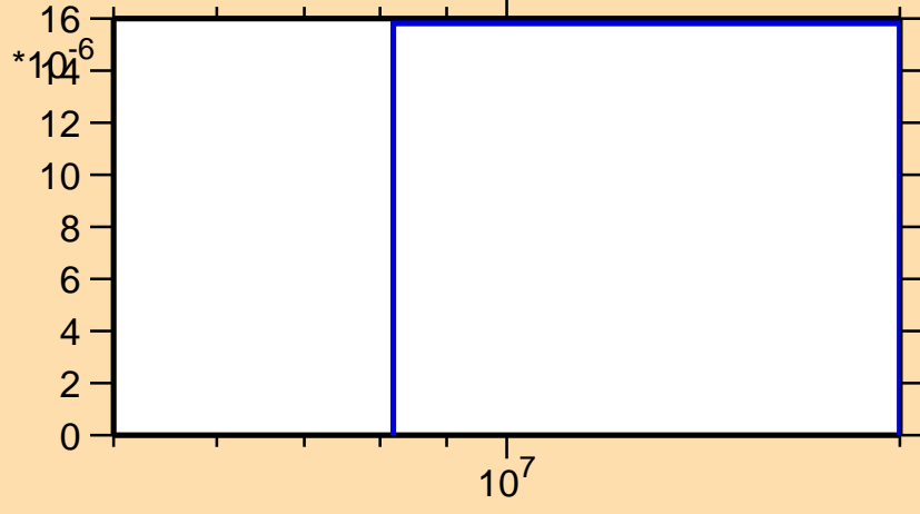
\sigma vs. E for ^{151}\text{Nd}(n,n\alpha)
