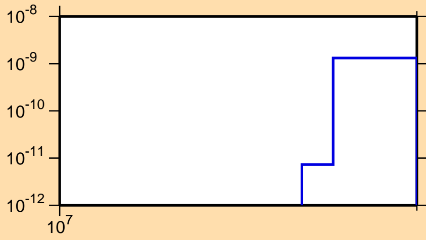
\sigma vs. E for ^{152}\text{Nd}(n,2n\alpha)
