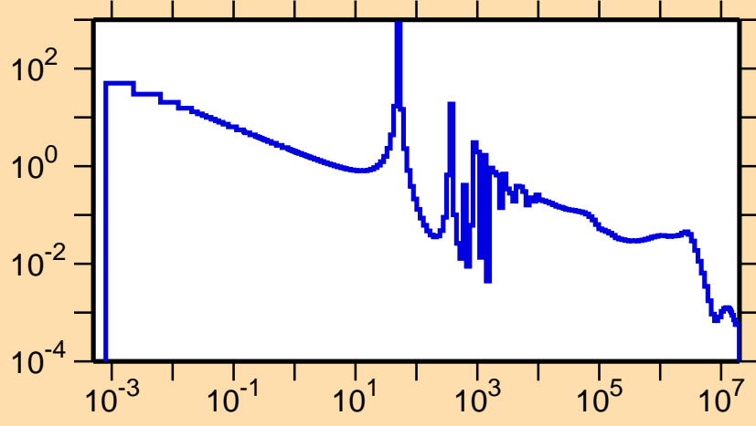
\sigma vs. E for ^{152}\text{Nd}(n,\gamma)
