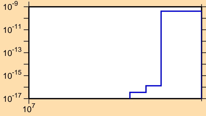
\sigma vs. E for ^{152}\text{Nd}(n,\text{nd})
