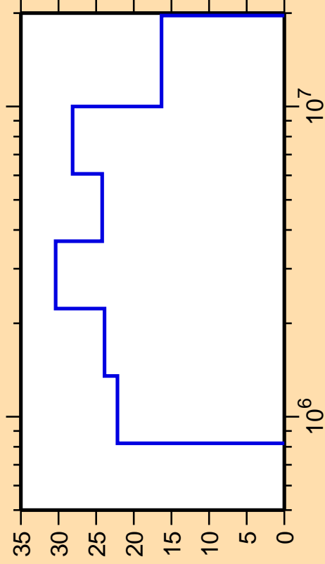
\Delta\sigma/\sigma vs. E for ^{152}\text{Nd}(n,n_4)
