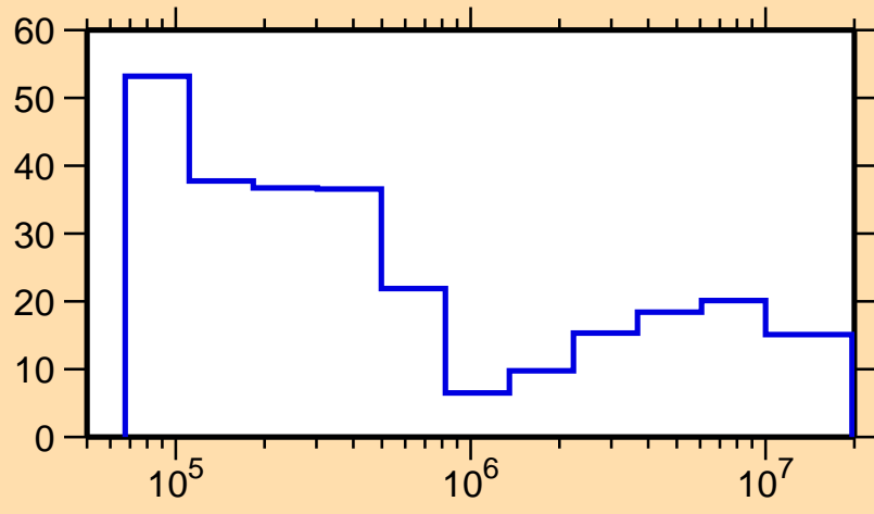
\Delta\sigma/\sigma vs. E for ^{152}\text{Nd}(n,n_1)
