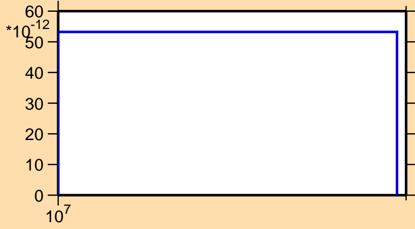
\sigma vs. E for ^{152}\text{Nd}(n,nt)
