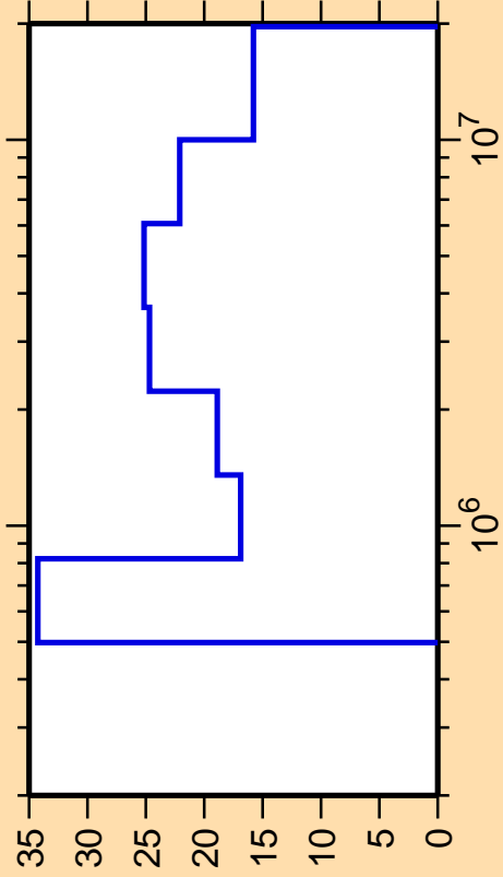
\Delta\sigma/\sigma vs. E for ^{152}\text{Nd}(n,n_3)
