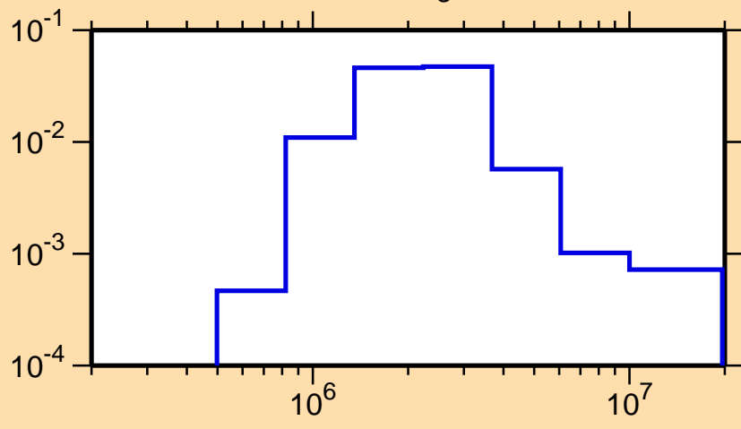
\sigma vs. E for ^{152}\text{Nd}(n,n_3)
