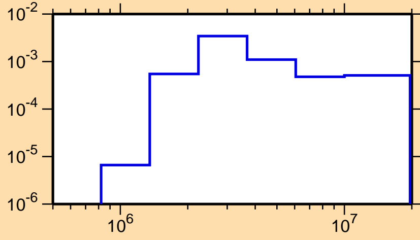
\sigma vs. E for ^{152}\text{Nd}(n,n_4)
