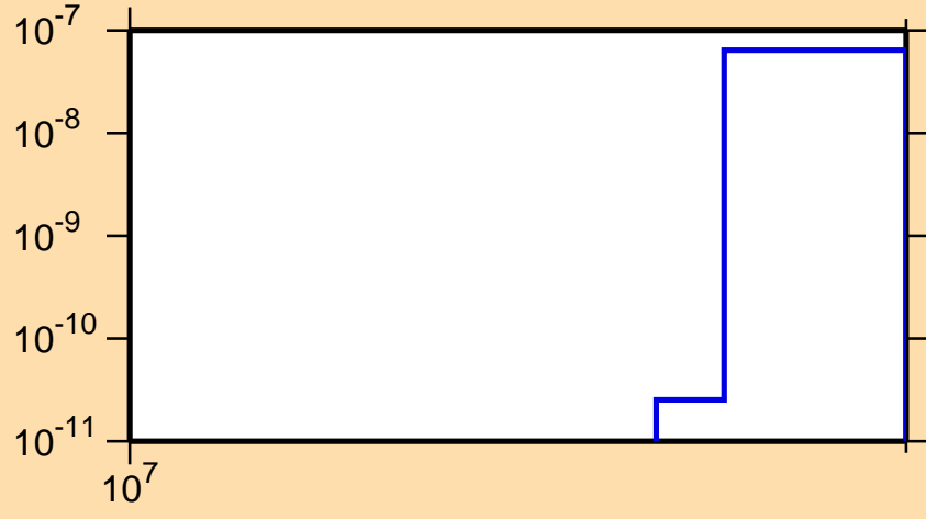
\sigma vs. E for ^{153}\text{Nd}(n,\text{nd})
