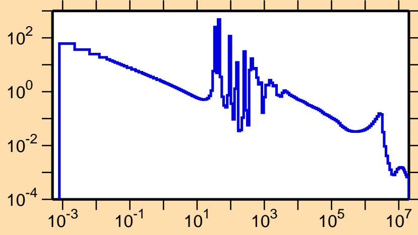
\sigma vs. E for ^{153}\text{Nd}(n,\gamma)
