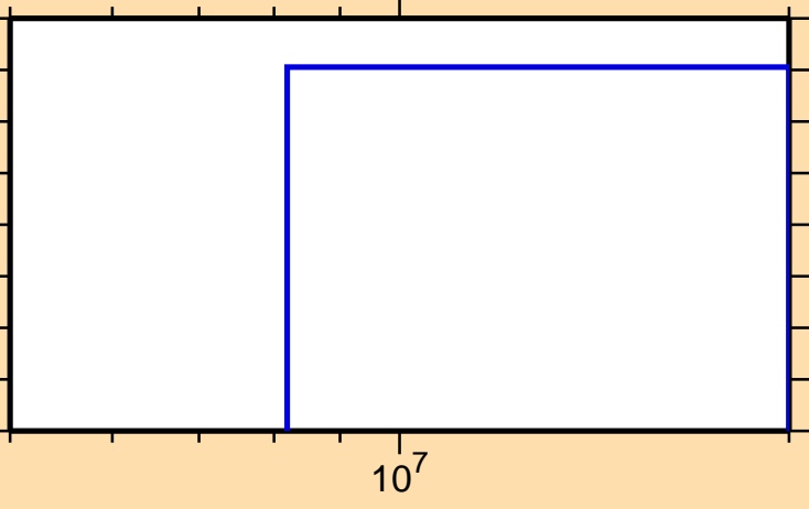
\sigma vs. E for ^{153}\text{Nd}(n,nt)
