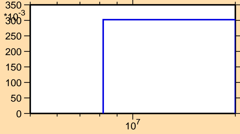
\sigma vs. E for ^{153}\text{Nd}(n,3n)
