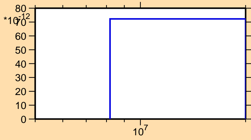
\sigma vs. E for ^{153}\text{Nd}(n,2n\alpha)
