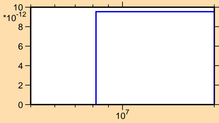
\sigma vs. E for ^{153}\text{Nd}(n,2np)
