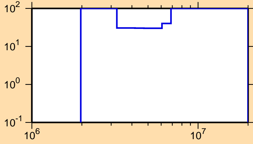
\Delta\sigma/\sigma vs. E for ^{154}\text{Nd}(n,n\text{cont.})
