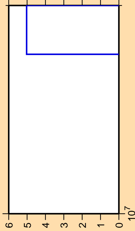
\Delta\sigma/\sigma vs. E for ^{154}\text{Nd}(n,2np)
