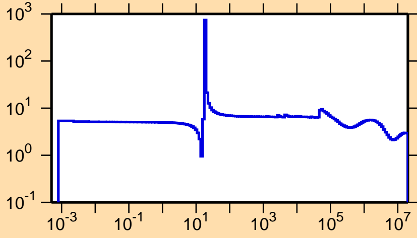
\sigma vs. E for ^{154}\text{Nd}(n,\text{el.})
