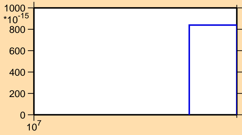
\sigma vs. E for ^{154}\text{Nd}(n,2np)
