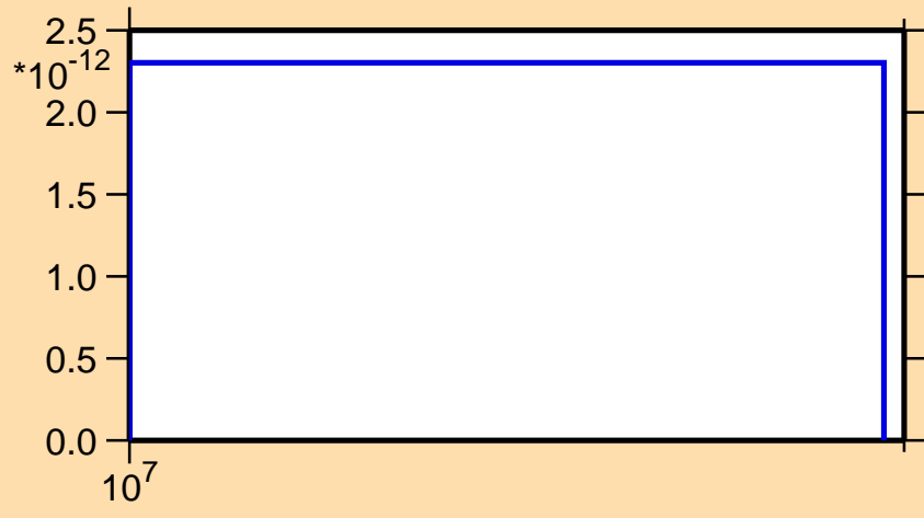
\sigma vs. E for ^{154}\text{Nd}(n,\text{nd})
