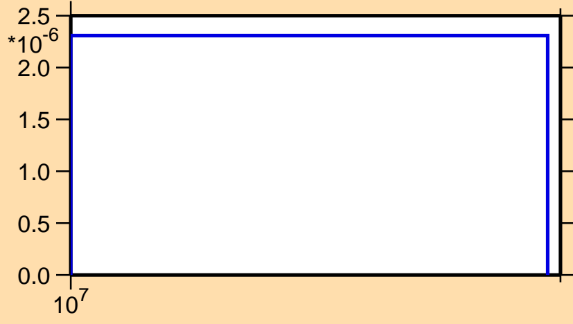
\sigma vs. E for ^{154}\text{Nd}(n,d)
