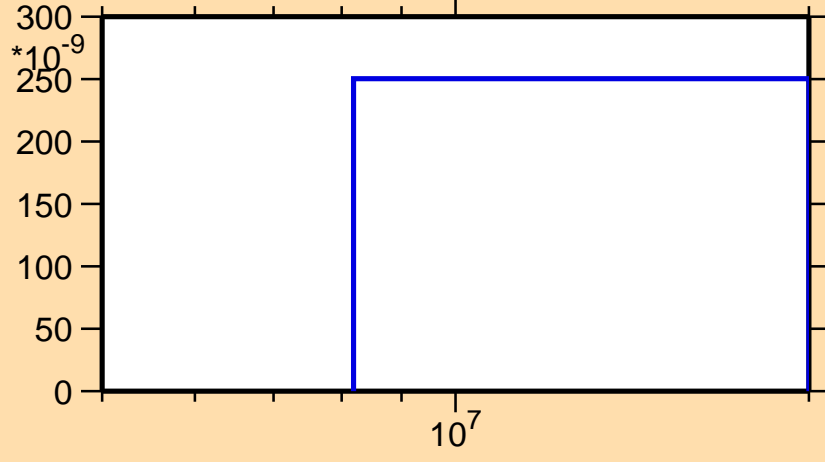
\sigma vs. E for ^{154}\text{Nd}(n,n\alpha)
