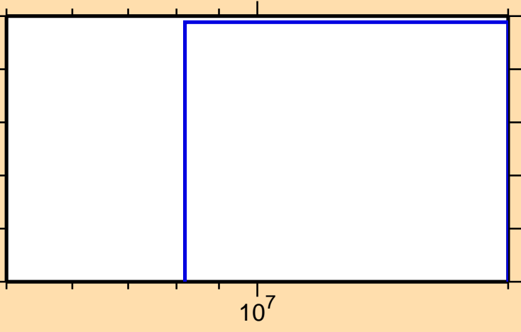
\sigma vs. E for ^{154}\text{Nd}(n,p)
