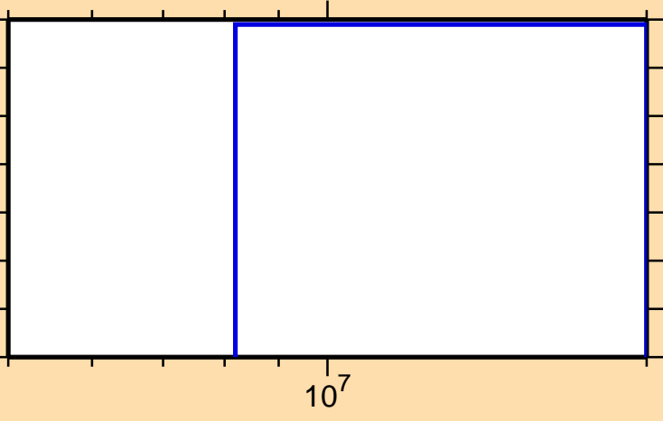
\sigma vs. E for ^{154}\text{Nd}(n,t)
