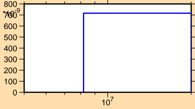
\sigma vs. E for ^{154}\text{Nd}(n,np)
