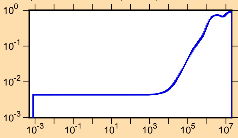
\mu vs. E for ^{155}\text{Nd}(\text{mt251})
