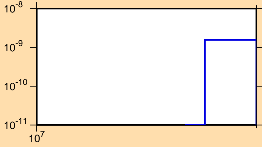
\sigma vs. E for ^{155}\text{Nd}(n,2n\alpha)
