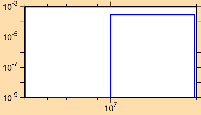
\sigma vs. E for ^{155}\text{Nd}(n,p)
