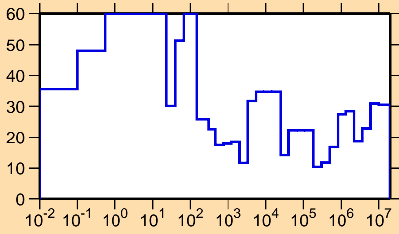
\Delta\sigma/\sigma vs. E for ^{155}\text{Nd}(n,\text{tot.})
