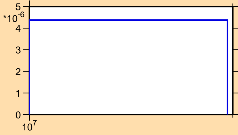
\sigma vs. E for ^{155}\text{Nd}(n,d)
