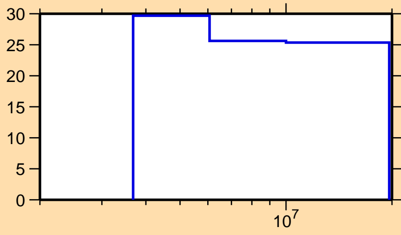
\Delta\sigma/\sigma vs. E for ^{155}\text{Nd}(n,2n)
