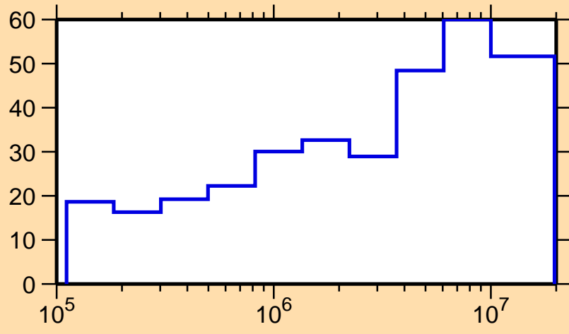
\Delta\sigma/\sigma vs. E for ^{155}\text{Nd}(n,\text{el.})
