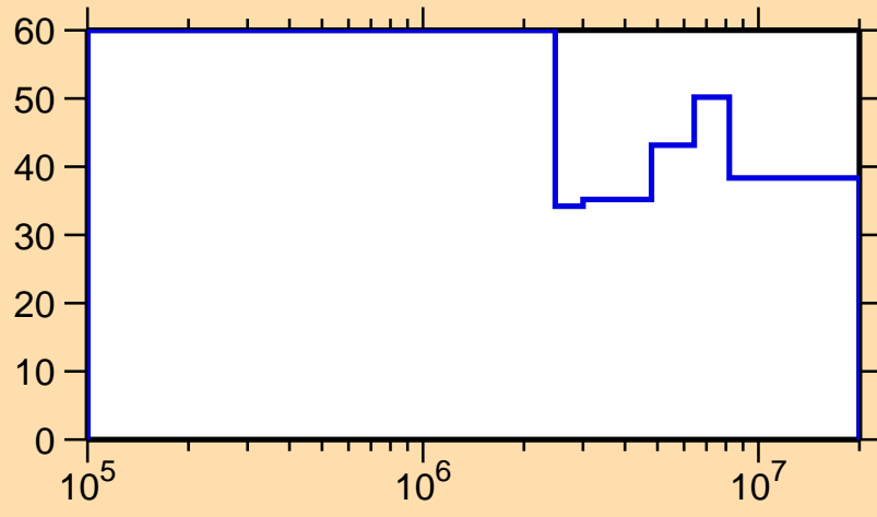
\Delta\sigma/\sigma vs. E for ^{155}\text{Nd}(n,n_1)
