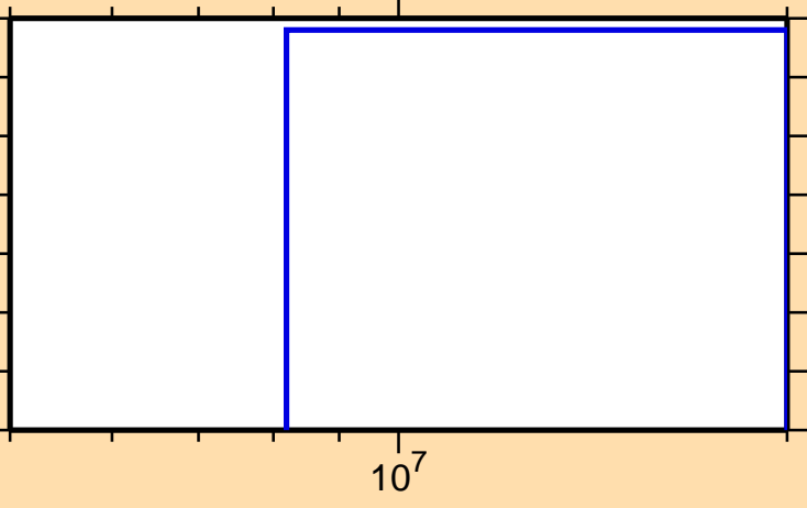
\sigma vs. E for ^{155}\text{Nd}(\text{mt } 11)
