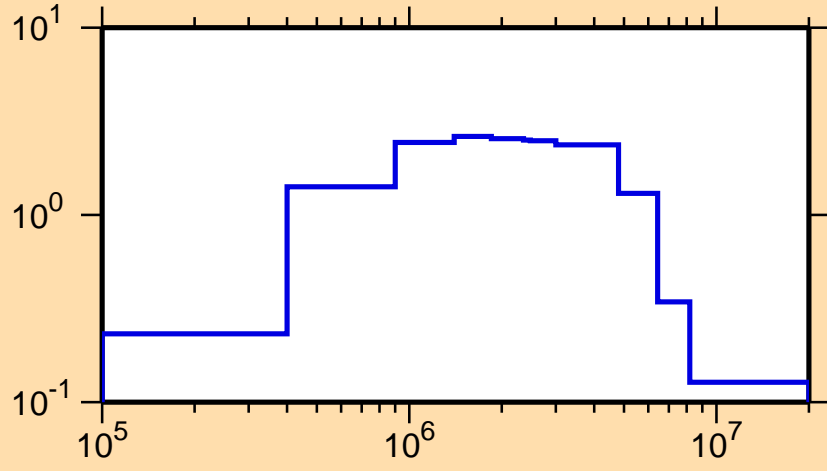
\sigma vs. E for ^{155}\text{Nd}(n,\text{inel.})
