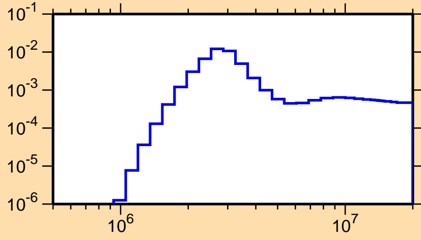
\sigma vs. E for ^{156}\text{Nd}(n,n_4)
