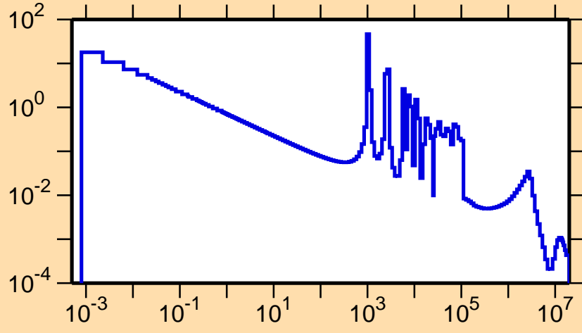
\sigma vs. E for ^{156}\text{Nd}(n,\gamma)
