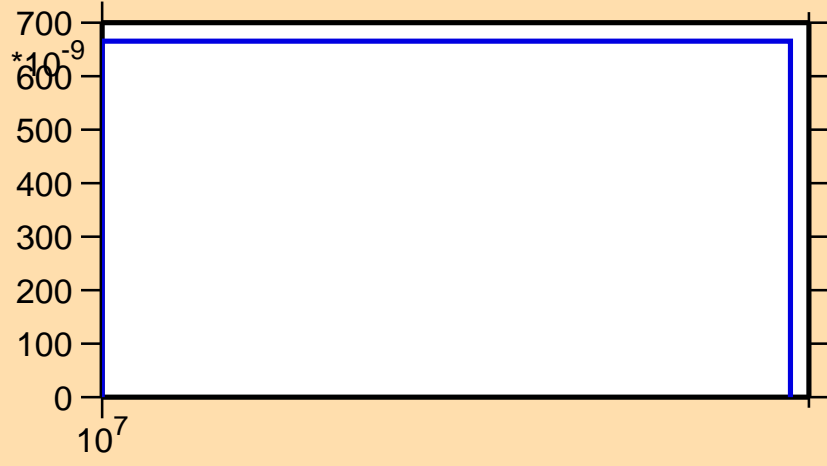
\sigma vs. E for ^{156}\text{Nd}(n,d)
