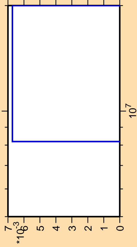
\Delta\sigma/\sigma vs. E for ^{156}\text{Nd}(n,2np)
