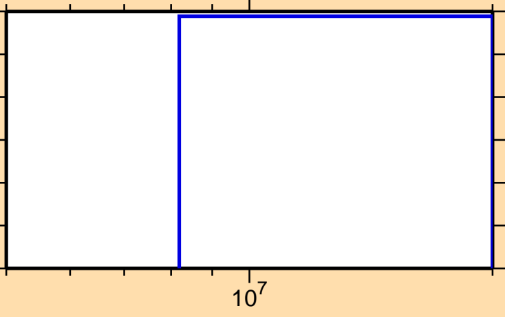
\sigma vs. E for ^{156}\text{Nd}(n,t)
