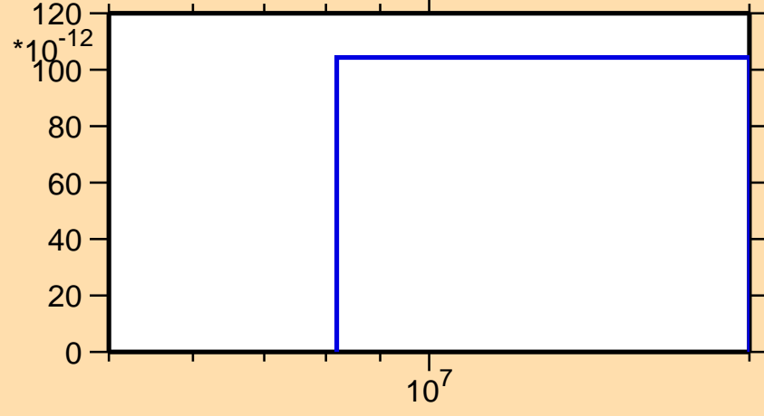
\sigma vs. E for ^{156}\text{Nd}(n,nt)
