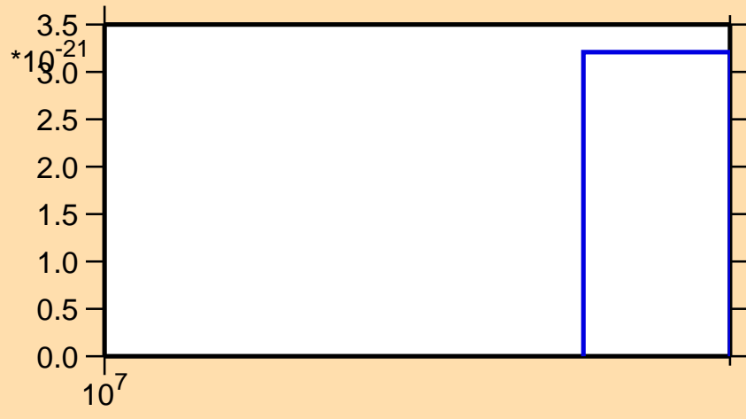
\sigma vs. E for ^{157}\text{Nd} (mt 11)
