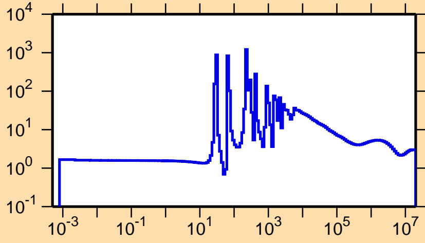
\sigma vs. E for ^{157}\text{Nd}(n,\text{el.})
