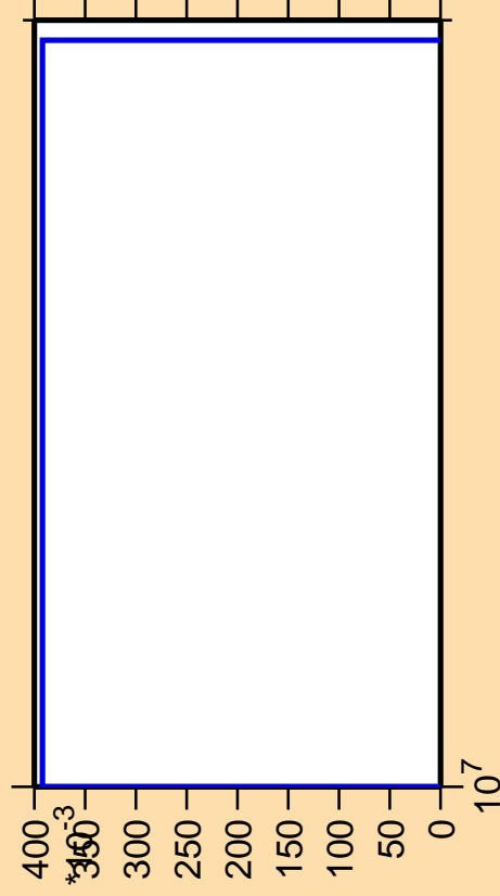
\Delta\sigma/\sigma vs. E for ^{157}\text{Nd}(n,2np)
