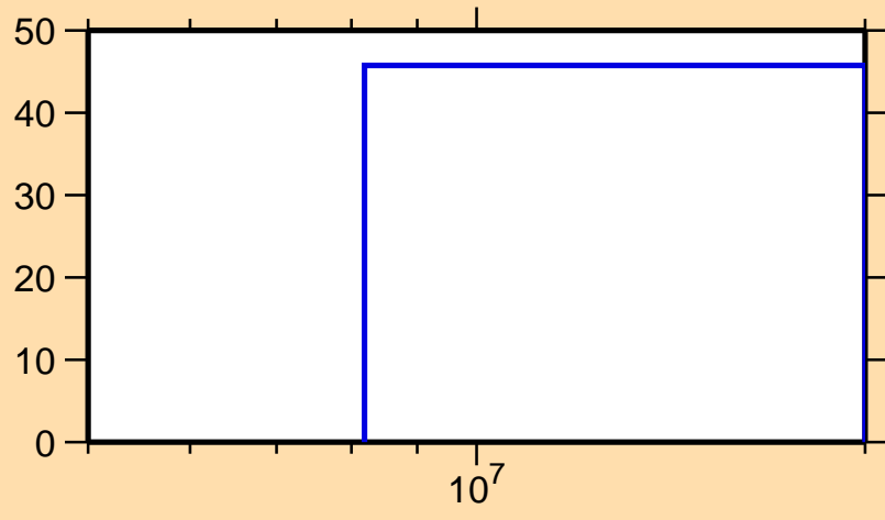
\Delta\sigma/\sigma vs. E for ^{157}\text{Nd}(n,ncont.)
