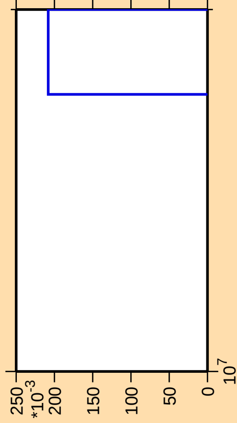
\Delta\sigma/\sigma vs. E for ^{18}\text{Ne}(n,\text{nd})
