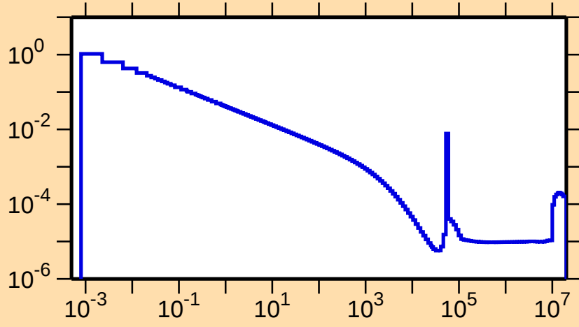
\sigma vs. E for ^{18}\text{Ne}(n,\gamma)
