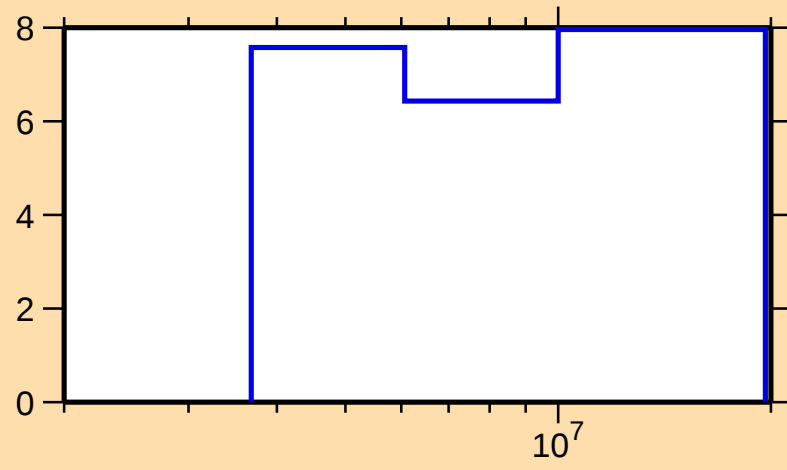
\Delta\sigma/\sigma vs. E for ^{18}\text{Ne}(n,n\text{nonel.})
