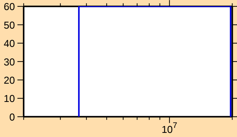
\Delta\sigma/\sigma vs. E for ^{18}\text{Ne}(n,n\text{cont.})
