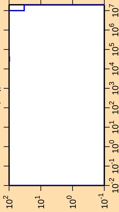
\Delta\sigma/\sigma vs. E for ^{18}\text{Ne}(n,\gamma)
