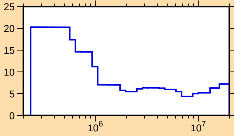
\Delta\sigma/\sigma vs. E for ^{19}\text{Ne}(n,\text{nonel.})
