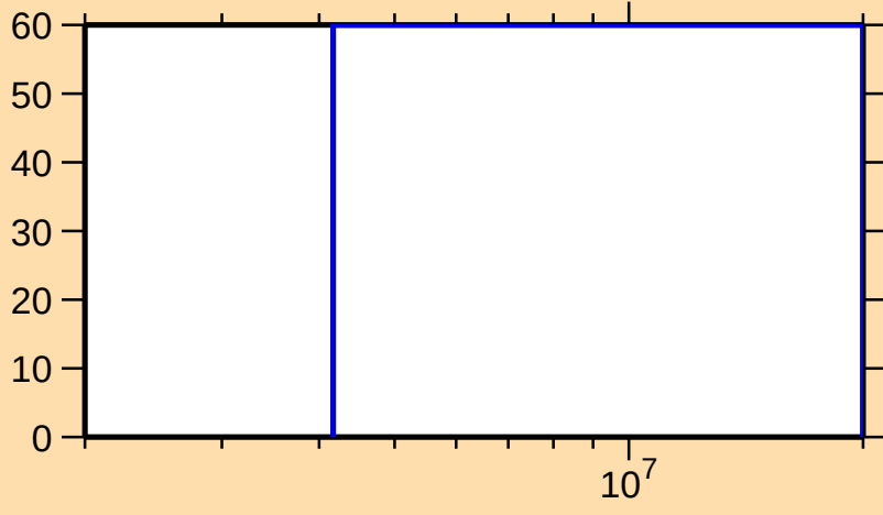
\Delta\sigma/\sigma vs. E for ^{19}\text{Ne}(n,n\text{cont.})
