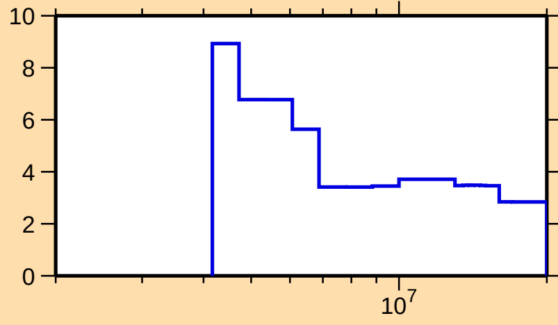
\Delta\sigma/\sigma vs. E for ^{19}\text{Ne}(n,\text{tot.})
