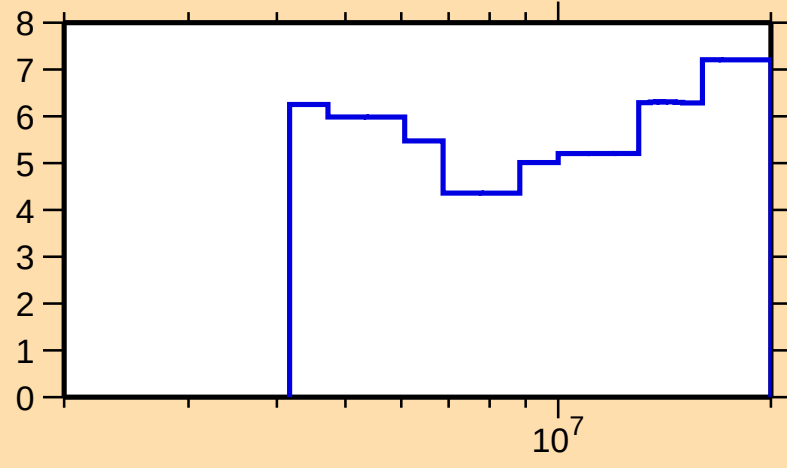
\Delta\sigma/\sigma vs. E for ^{19}\text{Ne}(n,n\text{oncl.})
