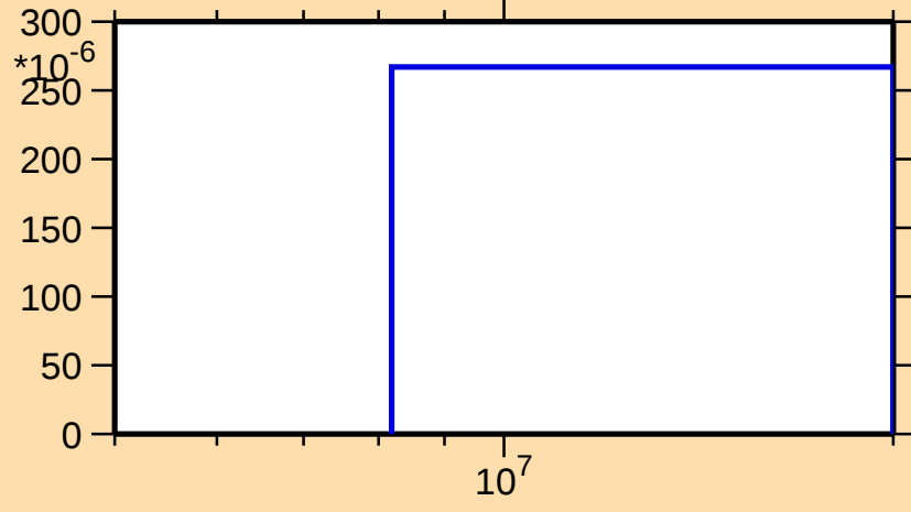
\sigma vs. E for ^{19}\text{Ne}(\text{mt } 45)
