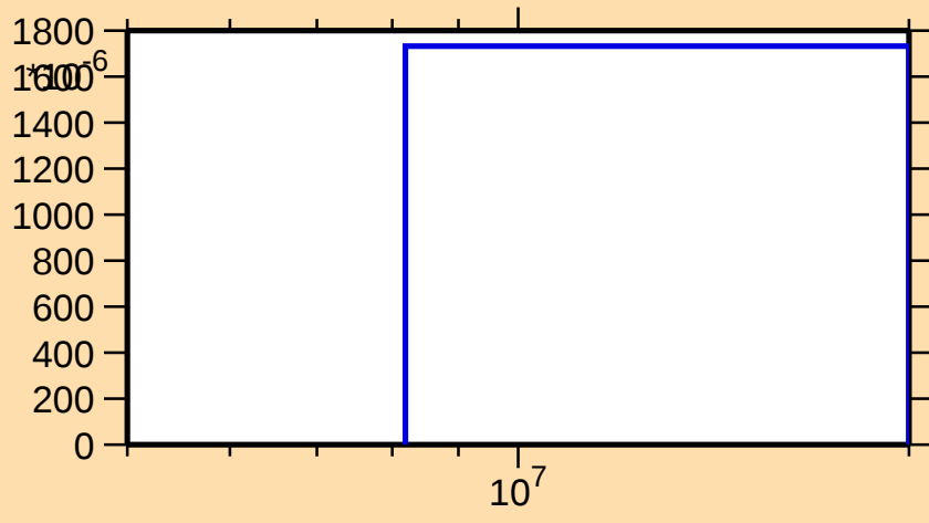
\sigma vs. E for ^{19}\text{Ne}(\text{mt } 34)
