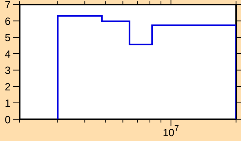
\Delta\sigma/\sigma vs. E for ^{19}\text{Ne}(n,n\text{onel.})
