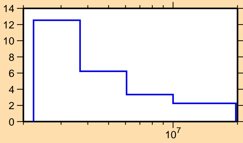
\Delta\sigma/\sigma vs. E for ^{20}\text{Ne}(n,\text{tot.})
