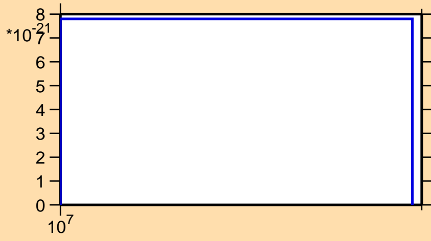
\sigma vs. E for ^{20}\text{Ne}(n,\text{pd})
