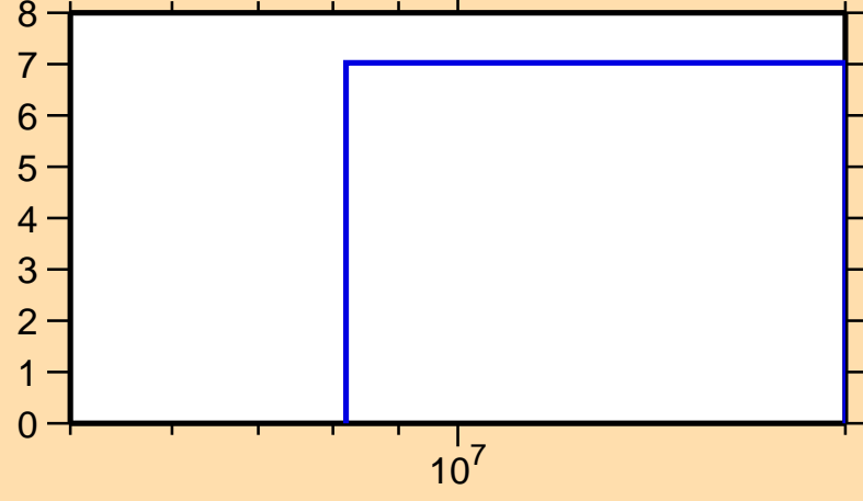
\Delta\sigma/\sigma vs. E for ^{20}\text{Ne}(n,\text{el.})
