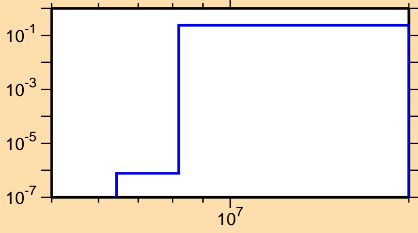
\sigma vs. E for ^{20}\text{Ne}(n,n\alpha)
