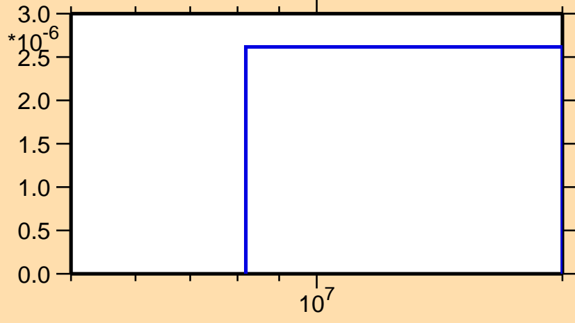
\sigma vs. E for ^{20}\text{Ne}(n,t)
