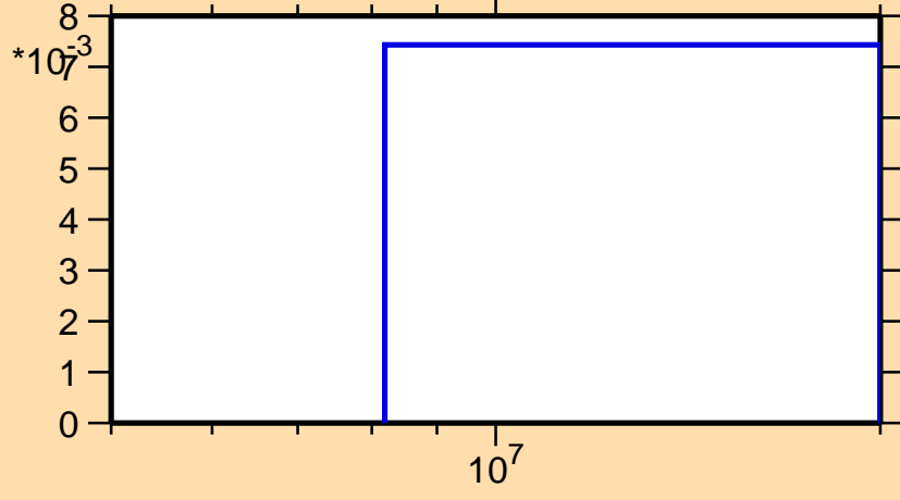
\sigma vs. E for ^{20}\text{Ne}(n,d)
