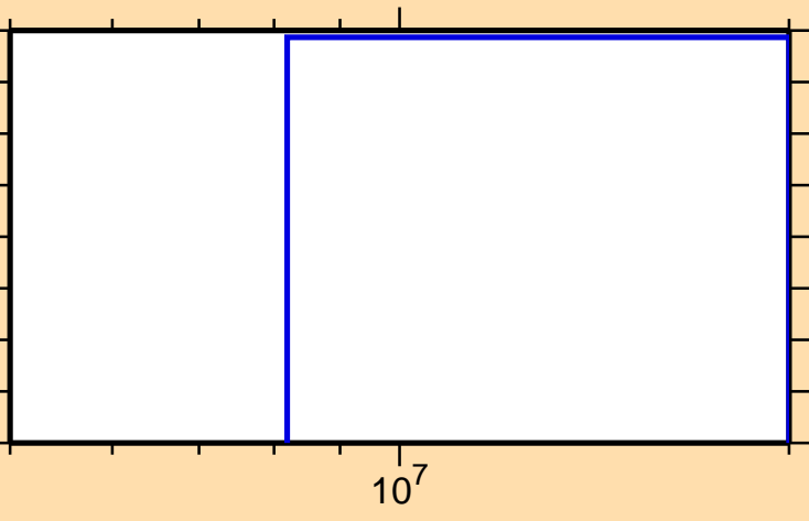
\sigma vs. E for ^{20}\text{Ne}(\text{mt } 45)
