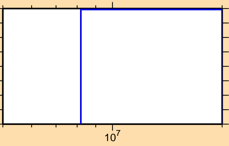
\sigma vs. E for ^{20}\text{Ne}(n,p\alpha)
