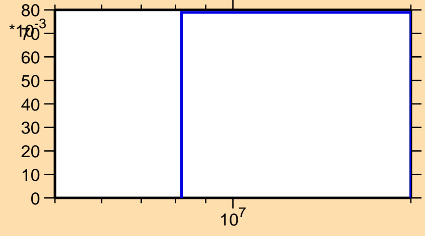
\sigma vs. E for ^{20}\text{Ne}(n,n\text{cont.})
