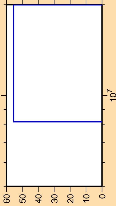
\Delta\sigma/\sigma vs. E for ^{20}\text{Ne}(\text{mt } 45)
