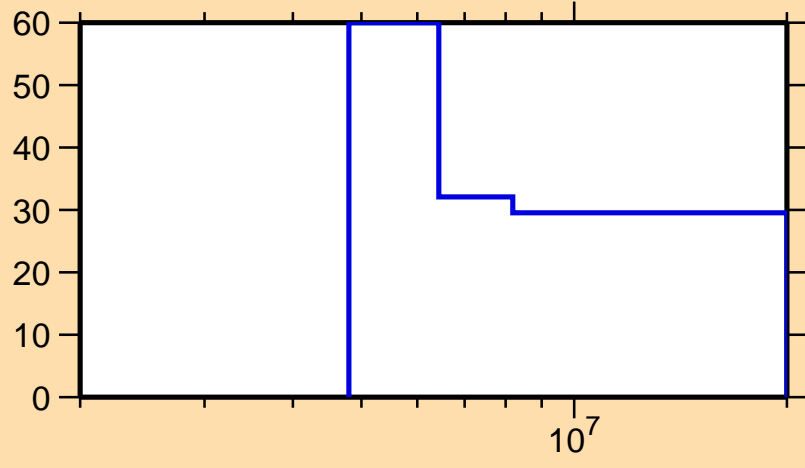
\Delta\sigma/\sigma vs. E for ^{21}\text{Ne}(n,p)
