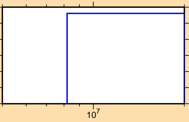
\sigma vs. E for ^{21}\text{Ne}(n,2n\alpha)
