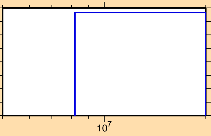
\sigma vs. E for ^{21}\text{Ne}(n,np)
