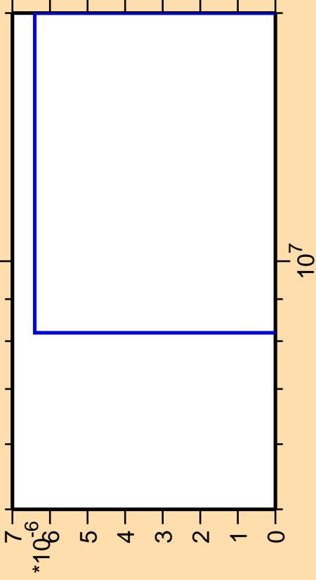
\Delta\sigma/\sigma vs. E for ^{21}\text{Ne}(n,\text{pt})
