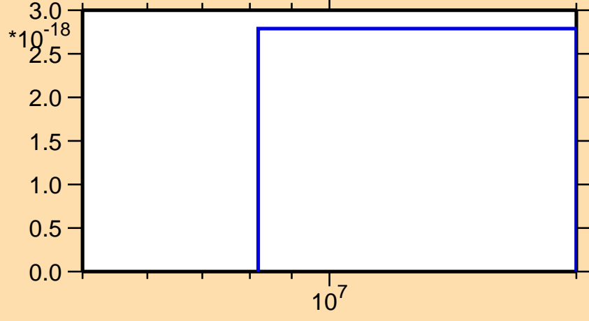
\sigma vs. E for ^{21}\text{Ne}(n,\text{pt})
