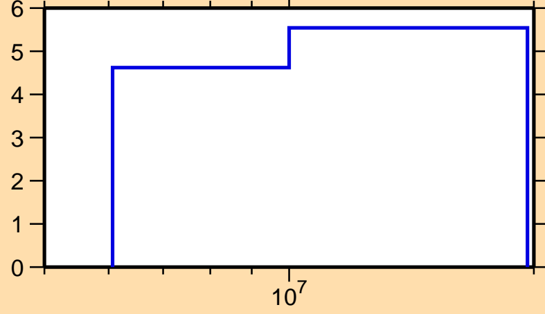
\Delta\sigma/\sigma vs. E for ^{22}\text{Ne}(n,\text{inel.})
