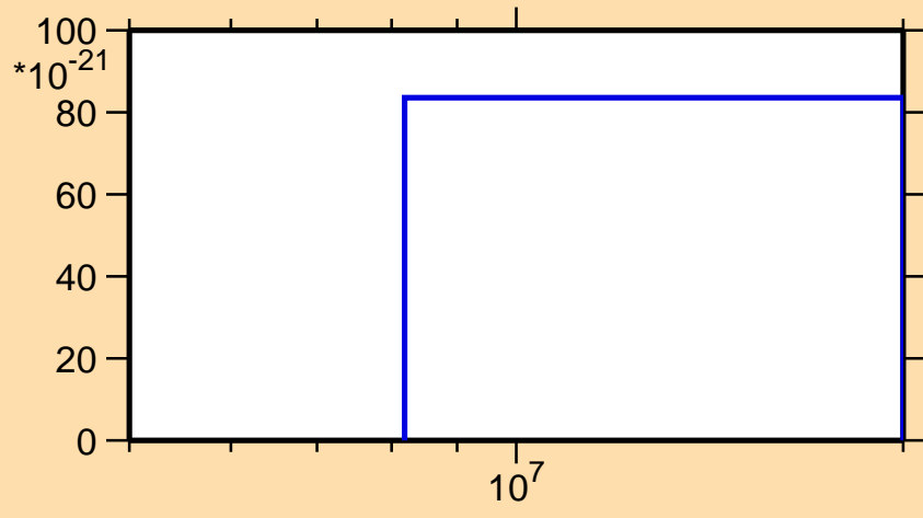
\sigma vs. E for ^{22}\text{Ne}(n,\text{He}3)
