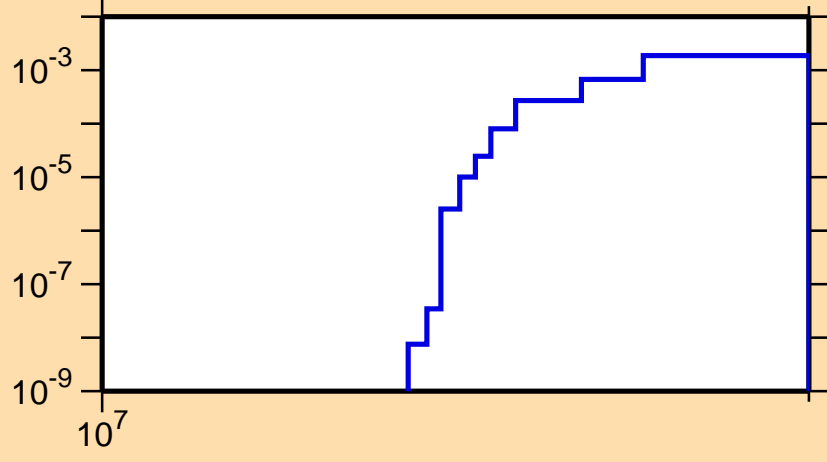
\sigma vs. E for ^{23}\text{Ne}(n,d)
