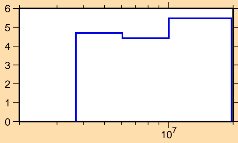
\Delta\sigma/\sigma vs. E for ^{23}\text{Ne}(n,n\text{nonel.})
