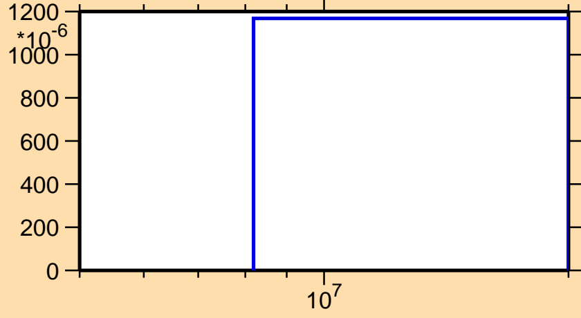
\sigma vs. E for ^{23}\text{Ne}(n,n\alpha)
