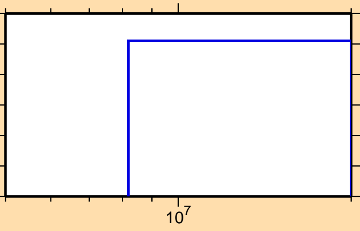
\sigma vs. E for ^{23}\text{Ne}(n,3n)
