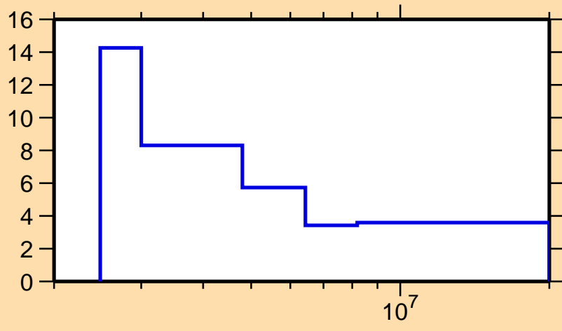
\Delta\sigma/\sigma vs. E for ^{23}\text{Ne}(n,\text{tot.})
