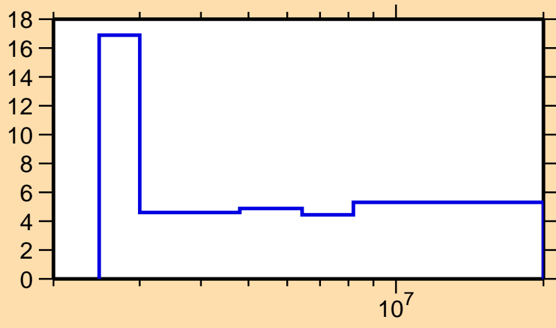
\Delta\sigma/\sigma vs. E for ^{23}\text{Ne}(n,\text{nonel.})
