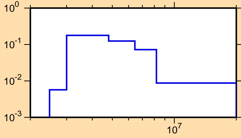
\sigma vs. E for ^{23}\text{Ne}(n,n_2)
