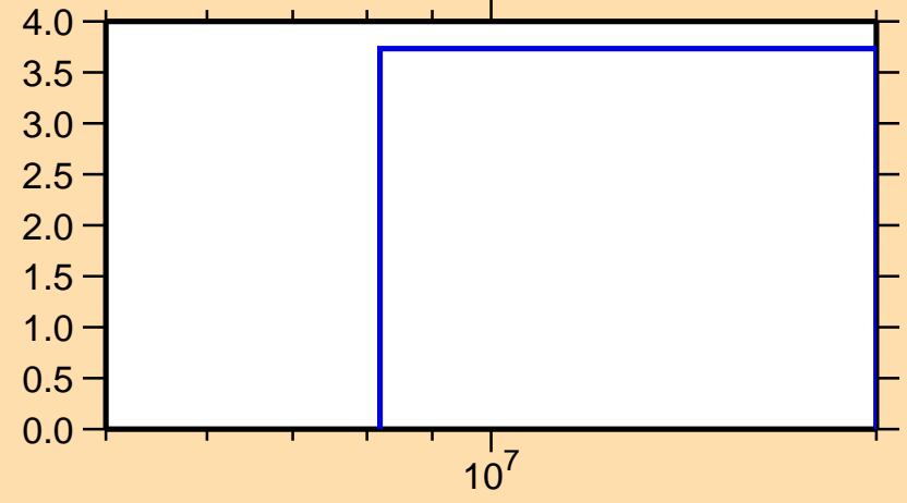
\Delta\sigma/\sigma vs. E for ^{24}\text{Ne}(n,2n)
