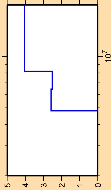
\Delta\sigma/\sigma vs. E for ^{24}\text{Ne}(n,n_4)
