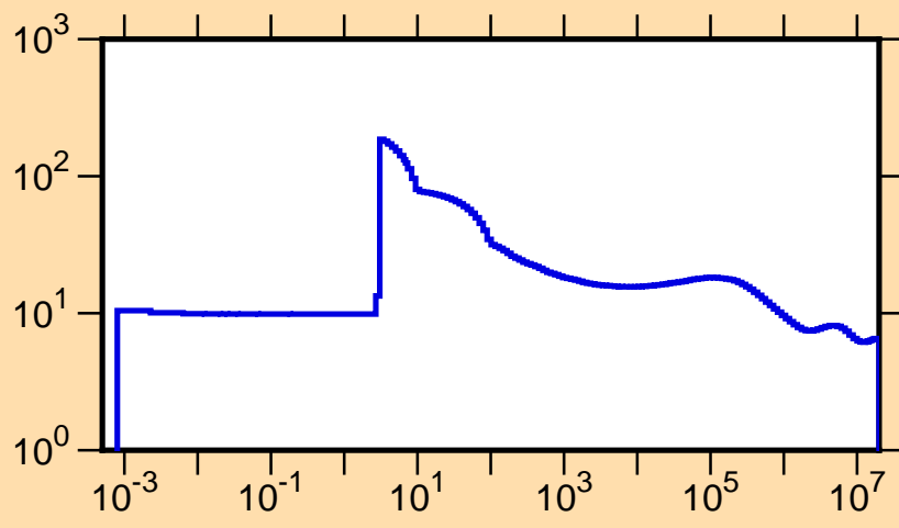
\sigma vs. E for ^{284}
