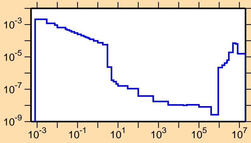
\sigma vs. E for ^{284}\gamma
