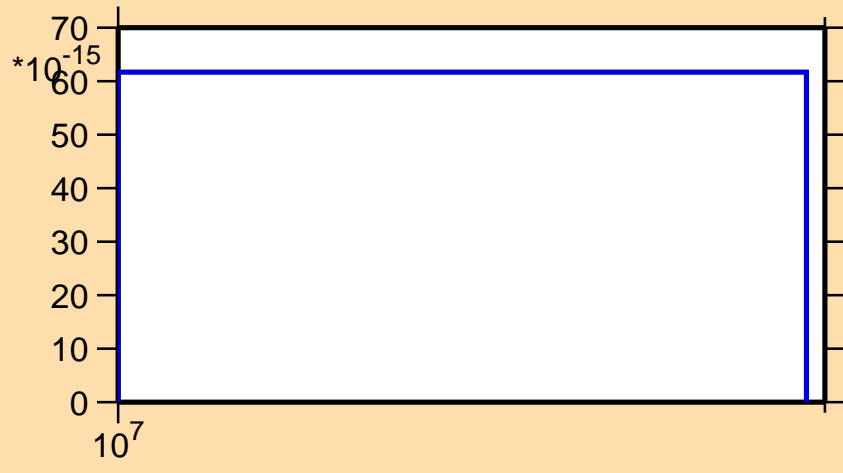
\sigma vs. E for ^{285}\text{He3}
