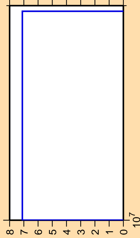
\Delta\sigma/\sigma vs. E for ^{286}\text{He3} )
