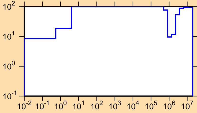
\Delta\sigma/\sigma vs. E for ^{286}\gamma
