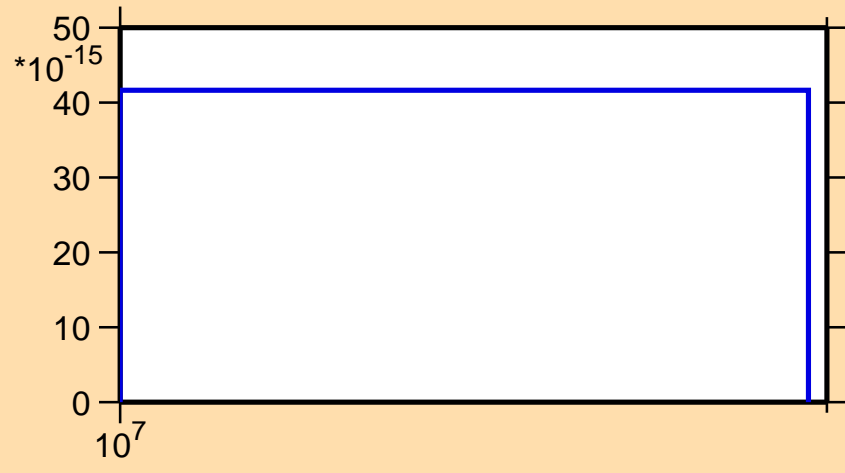
\sigma vs. E for ^{287}
