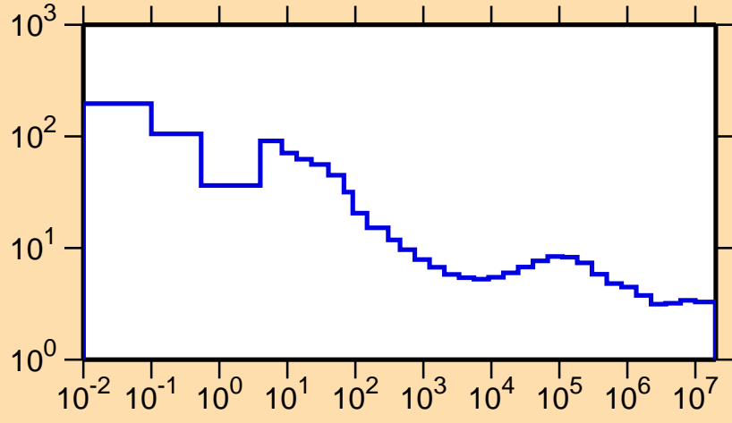
\sigma vs. E for ^{287}
