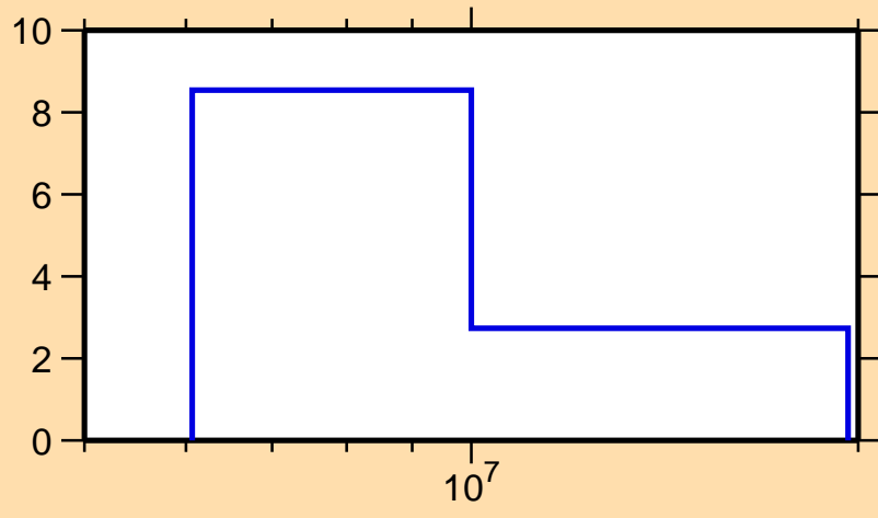
\Delta\sigma/\sigma vs. E for 287
