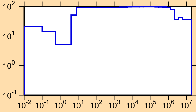
\Delta\sigma/\sigma vs. E for ^{287}\gamma
