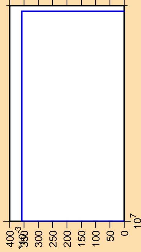
\Delta\sigma/\sigma vs. E for ^{287}\text{He3}
