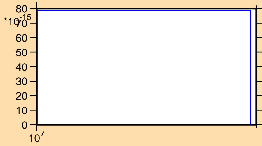
\sigma vs. E for ^{287}\text{He3}
