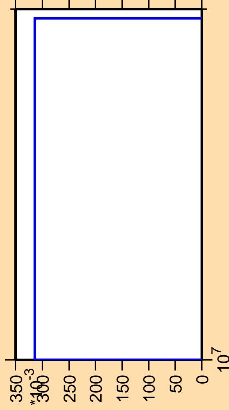
\Delta\sigma/\sigma vs. E for ^{287}
