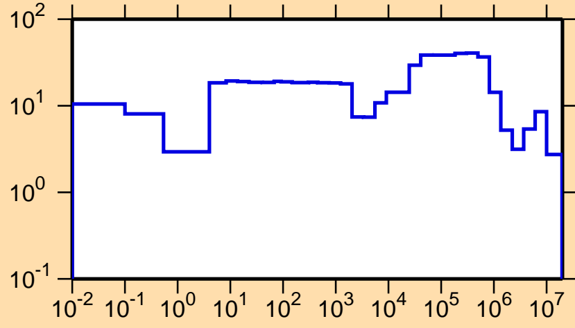
\Delta\sigma/\sigma vs. E for ^{287}
