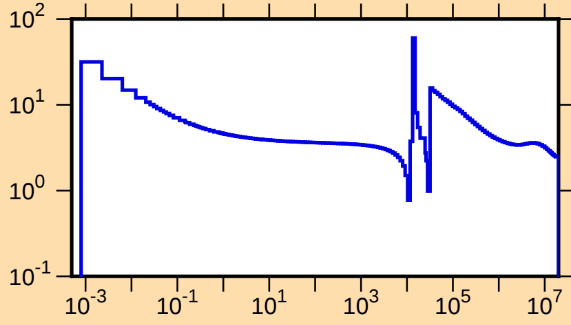
\sigma vs. E for ^{56}\text{Ni}(n,\text{tot.})
