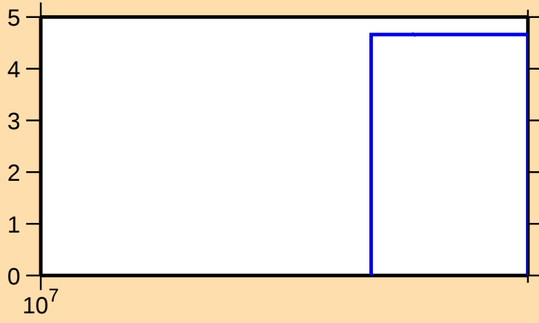
\Delta\sigma/\sigma vs. E for ^{56}\text{Ni}(n,\text{el.})
