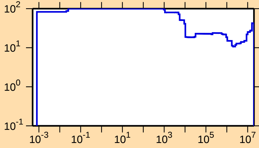
\Delta\sigma/\sigma vs. E for ^{56}\text{Ni}(n,p)
