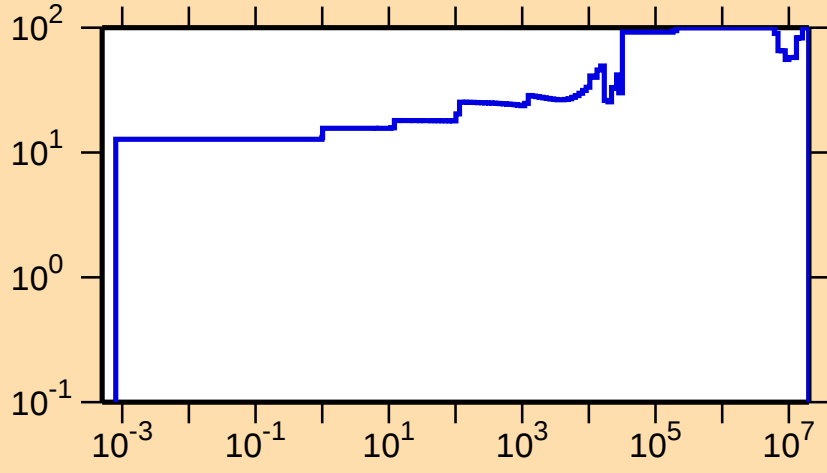
\Delta\sigma/\sigma vs. E for ^{56}\text{Ni}(n,\gamma)
