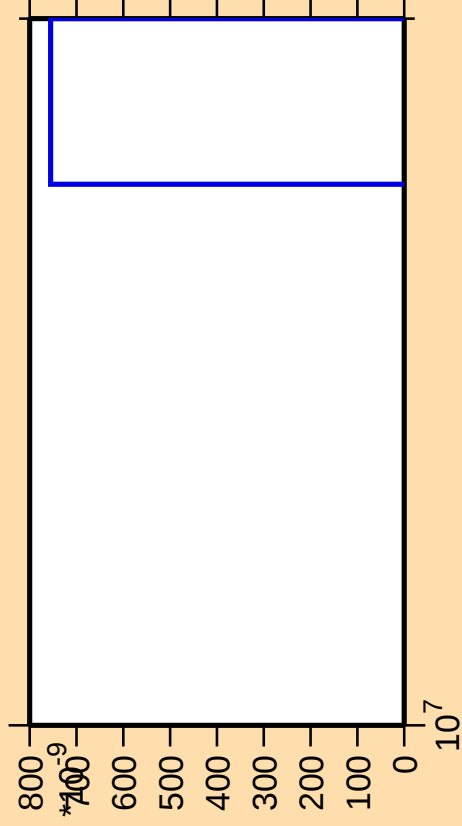
\Delta\sigma/\sigma vs. E for ^{56}\text{Ni}(\text{mt } 34)
