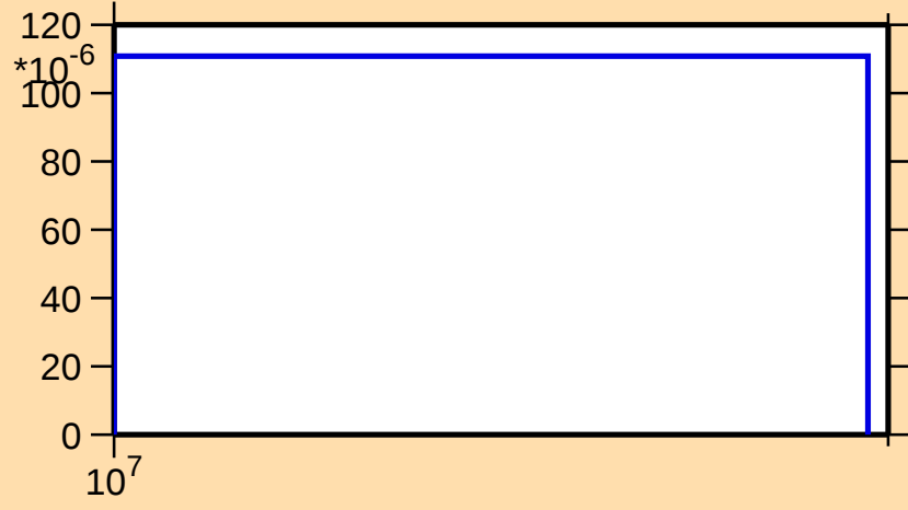
\sigma vs. E for ^{56}\text{Ni}(n,\text{pd})
