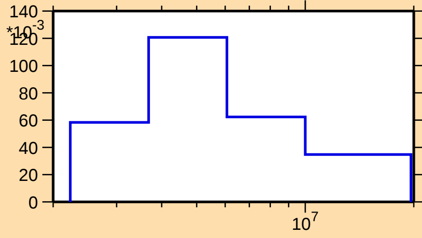
\sigma vs. E for ^{56}\text{Ni}(n,n_1)
