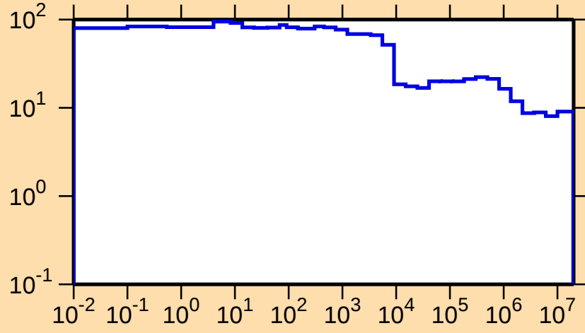
\Delta\sigma/\sigma vs. E for ^{56}\text{Ni}(n,\text{nonel.})
