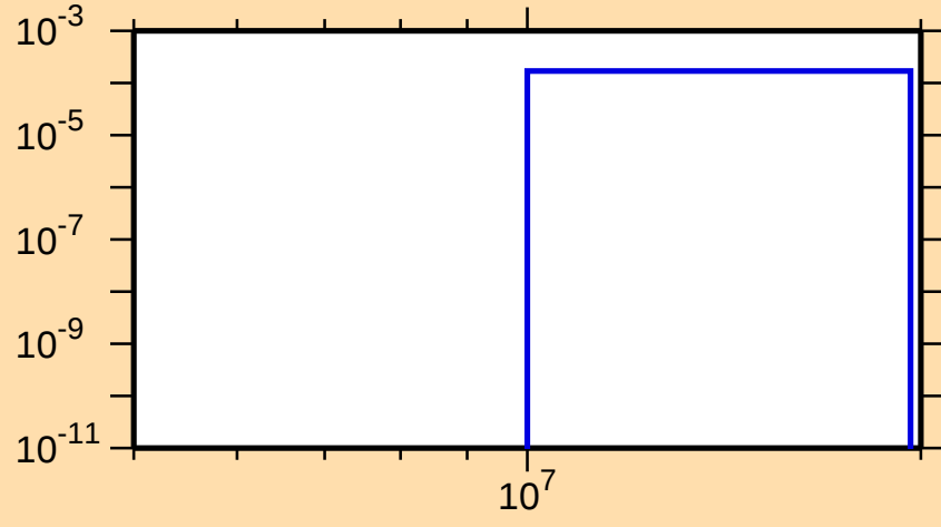
\sigma vs. E for ^{56}\text{Ni}(n,n\alpha)
