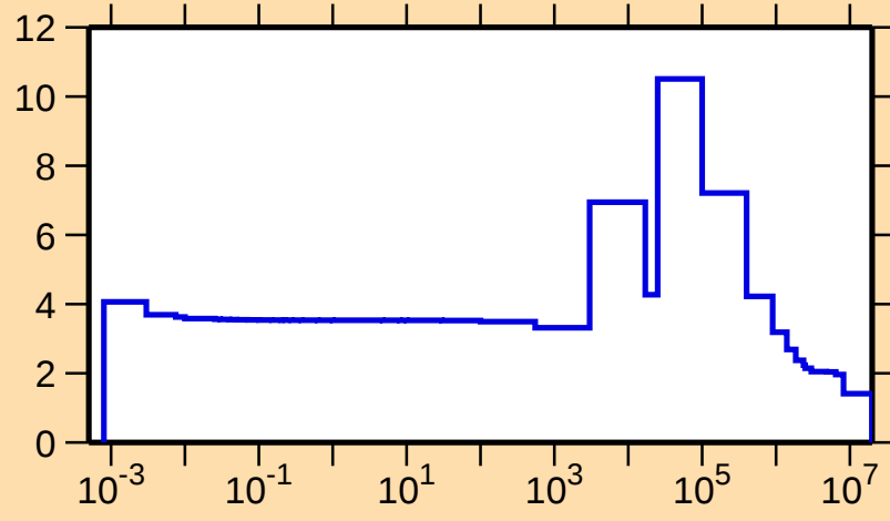
\sigma vs. E for ^{56}\text{Ni}(n,\text{el.})
