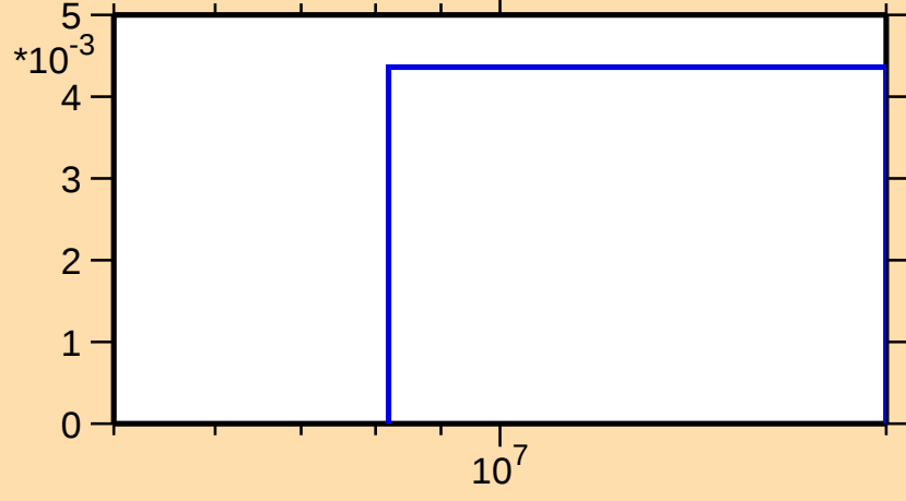
\sigma vs. E for ^{56}\text{Ni}(n,p\alpha)
