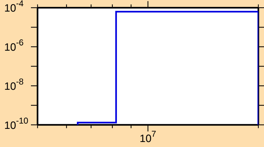
\sigma vs. E for ^{56}\text{Ni}(n,\text{He3})
