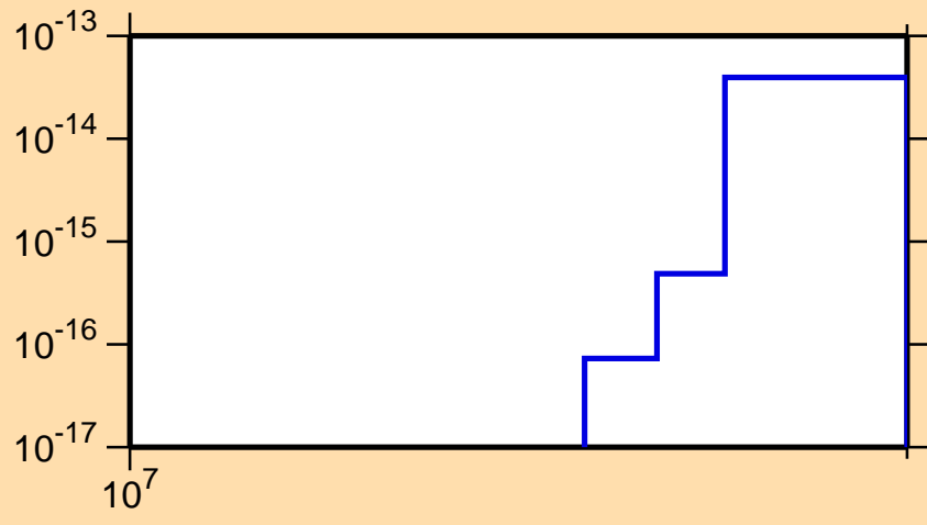
\sigma vs. E for ^{57}\text{Ni} (mt 45)
