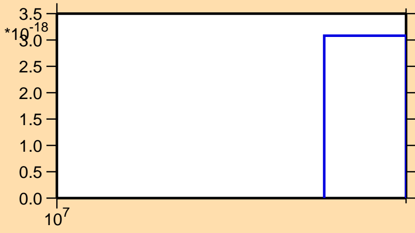
\sigma vs. E for ^{57}\text{Ni}(n,2n\alpha)
