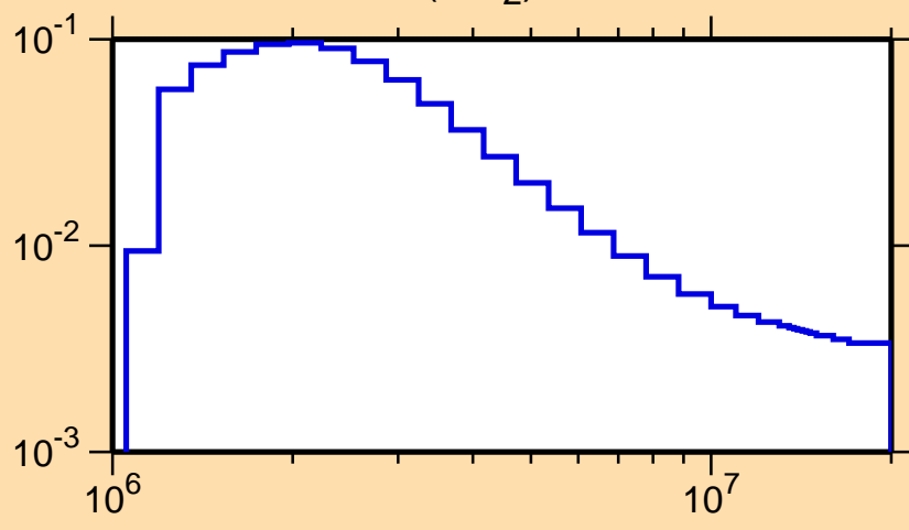
\sigma vs. E for ^{57}\text{Ni}(n,n_2)
