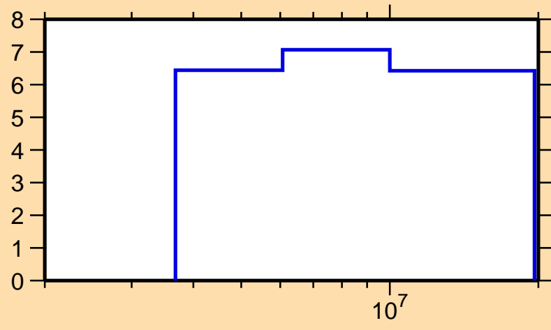
\Delta\sigma/\sigma vs. E for ^{57}\text{Ni}(n,n\text{nonel.})
