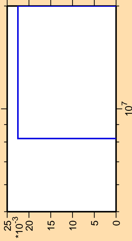
\Delta\sigma/\sigma vs. E for ^{57}\text{Ni}(\text{mt117})
