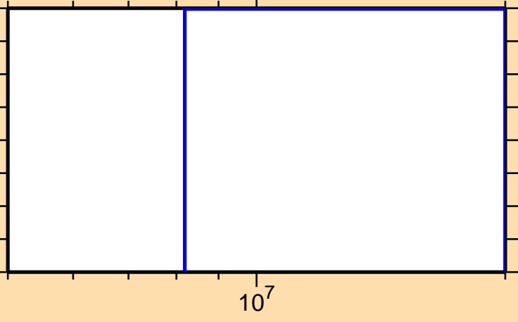
\sigma vs. E for ^{57}\text{Ni}(n,2np)
