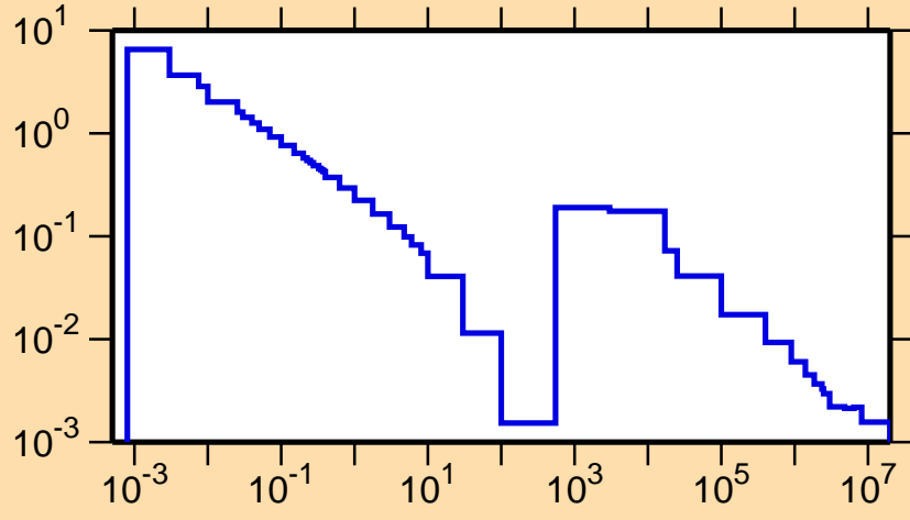
\sigma vs. E for ^{57}\text{Ni}(n,\gamma)
