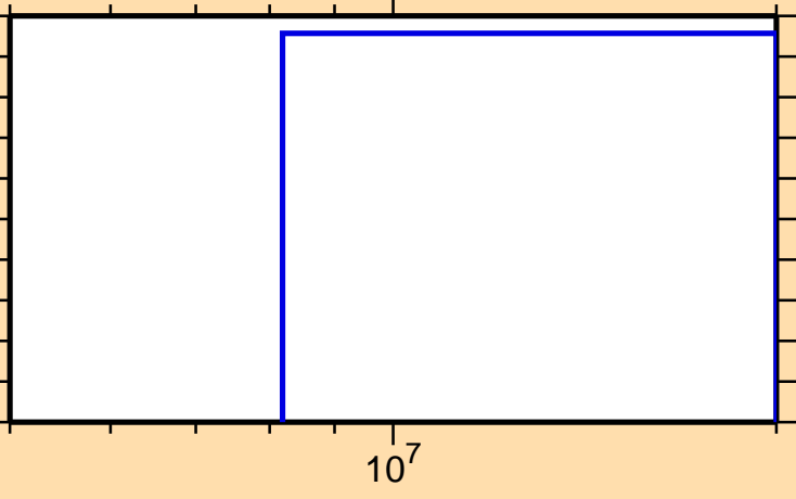
\sigma vs. E for ^{57}\text{Ni}(n,\text{pd})
