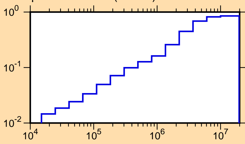
\mu vs. E for ^{58}\text{Ni}(\text{mt251})
