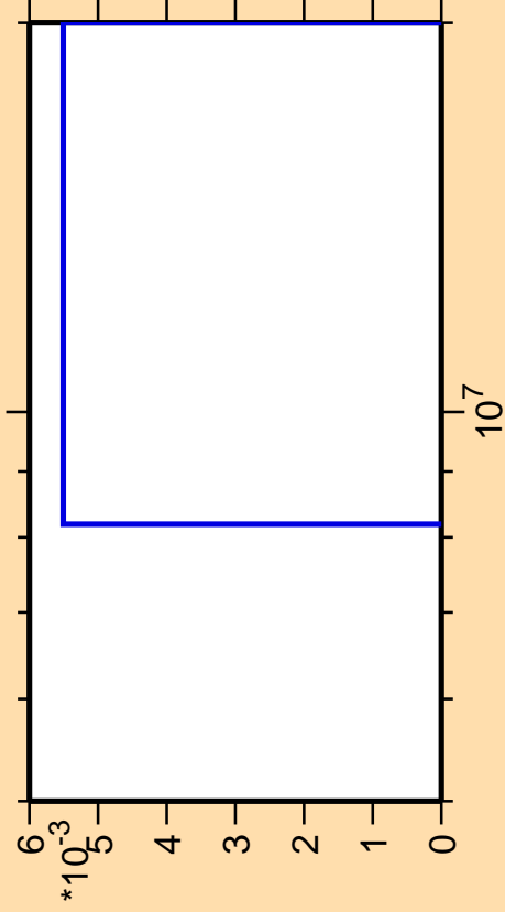
\Delta\sigma/\sigma vs. E for ^{58}\text{Ni}(\text{mt } 45)
