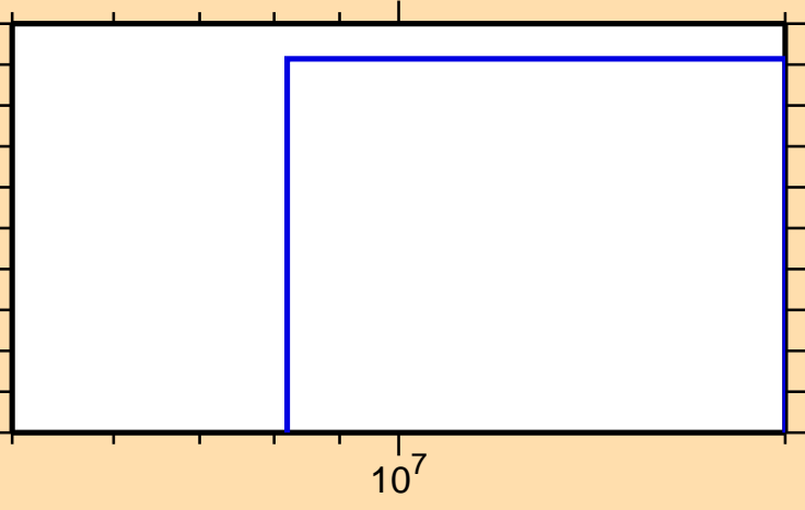
\sigma vs. E for ^{58}\text{Ni}(n,2n)
