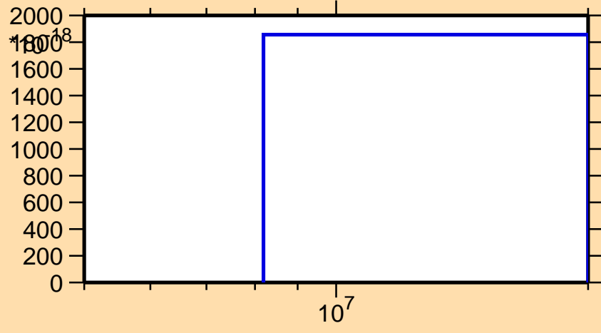
\sigma vs. E for ^{58}\text{Ni}(\text{mt } 45)
